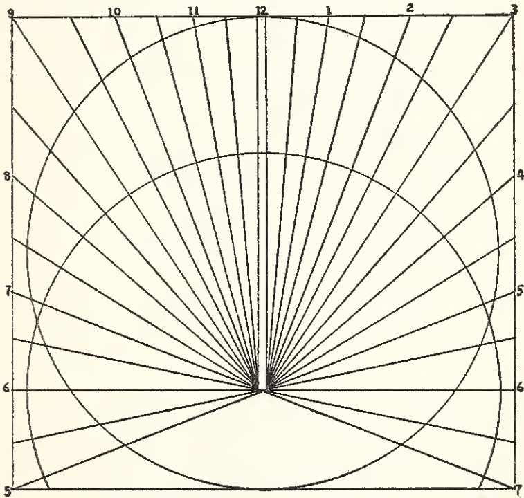
FIGURE 2.—Suggested forms for sundials
